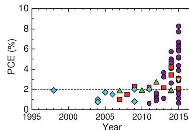
Fig. 2 Efficiency enhancement of polymer/polymer blend solar cells based on different polymer acceptors: cyanated phenylenevinylene-based polymers (diamonds); fluorene and BT-based polymers (triangles); thiazole-bridged diketopyrrolopyrrole-polymer (inverted triangle); 67 PDI-based polymers (squares); and NDI-based polymers (circles).
