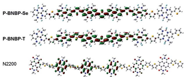
Fig. 2 Kohn-Sham LUMOs of model compounds of P-BNBP-Se, P-BNBP-T and N2200, based on calculations at the B3LYP/6-31G* level.
