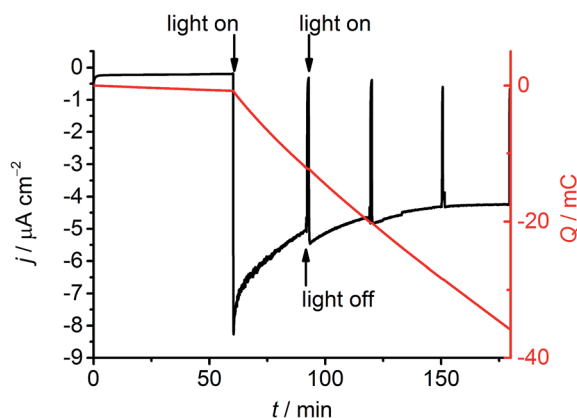
Fig. 5 CPPE of a NiO|RuP3-Zr 4+ -NiP photoelectrode (1 cm 2 ) at E_{\text{appl}} = 0.3 V vs. RHE in Na 2 SO 4 (0.5 M, pH 3) at room temperature. Electrolysis was performed in a 2-compartment PEC cell with the working and counter compartment separated by a Nafion membrane. The working electrode was held in the dark for 1 h, followed by irradiation for 2 h using a solar light simulator (100 mW cm -2 , AM1.5G filter, \lambda > 400 nm).
