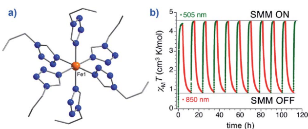
Fig. 8 (a) Molecular structure of [Fe(1-ptz) 6 ][(BF 4 ) 2 ] (2). Colour code: orange (Fe), blue (N), and grey (C). Hydrogen atoms omitted for clarity. (b) Excitation and de-excitation cycling between the HS and LS configuration of 2, represented as a variation in the \chi_M T product at 10 K, under a 5000 Oe field. Reprinted with permission from ref. 28. Copyright (2013) American Chemical Society.
