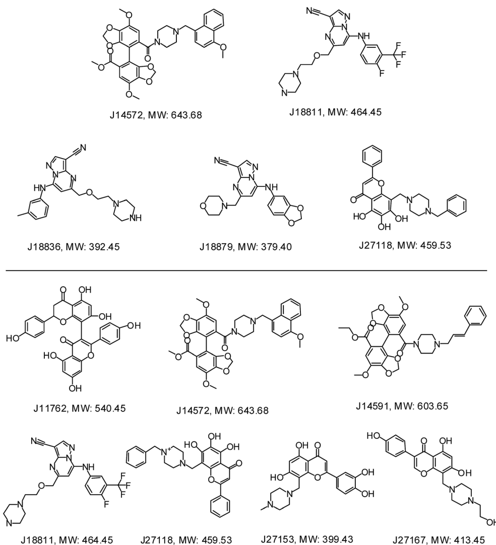
Fig. 9 Chemical structures of representative neuroprotective compounds against glutamate-induced (top) or \text{H}_2\text{O}_2 -induced (bottom) neurotoxicity in PC12 cell.
