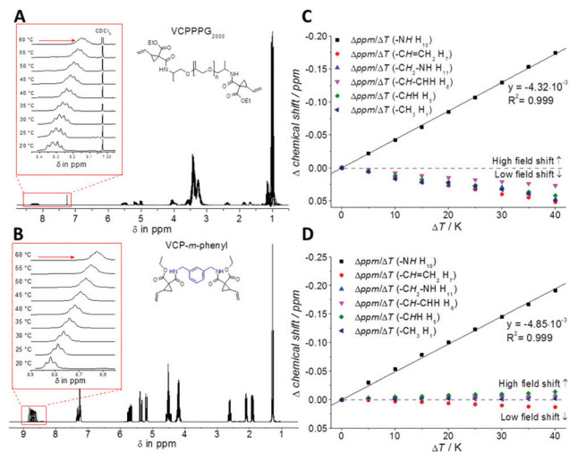
Fig. 2 (A + B) Variable-temperature ^1\text{H-NMR} experiments of VCP-PPG 2000 and VCP- m -phenyl (0.5 mM in \text{CDCl}_3 ) between 20–60 °C. (C + D) Graphical plot of chemical shift within ^1\text{H-NMR} experiments. With increased temperature a decreased deshielding effect is anticipated, as a partial rupture of the H-bonds occurs.
