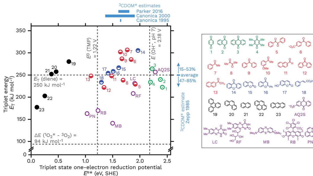
Fig. 8 Triplet energies ( E_T , \text{kJ mol}^{-1} ) vs. triplet state one-electron reduction potentials ( E^o ( {}^3\text{S}^*/\text{S}^- ), V SHE) for a selection of 23 DOM-like model compounds and a selection of widely used sensitizers. The horizontal lines correspond to the triplet excited state energy of a typical diene energy transfer probe and the singlet state energy of \text{O}_2 . The vertical lines correspond to the one-electron oxidation potentials of TMP, E^o(\text{ArOH}^{+}/\text{ArOH}) , and hydroxide at pH 7, E^o(\text{OH}^+/\text{OH}^-) . Selected estimates for {}^3\text{CDOM}^* values from Zepp, 9 Canonica, 79,106 and Parker and Mitch 48 are also shown. The data used for this figure is compiled in Table 1 along with the abbreviation definitions.
