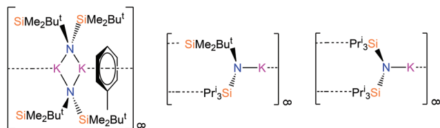
Fig. 1 The potassium silylamide complexes [\{\text{K}\{\mu\text{-N}(\text{SiMe}_2\text{Bu}^t)\}_2(\text{C}_7\text{H}_8)\}_\infty] , [\text{K}\{\text{N}(\text{SiPr}^i)_3(\text{SiMe}_2\text{Bu}^t)\}_\infty] and [\text{K}\{\text{N}(\text{SiPr}^i)_3\}_2]_\infty . 28
