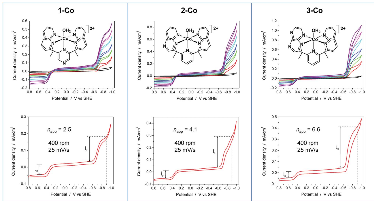
Fig. 6 RDEV of the series of cobalt catalysts. Panels: axial isomer 1-Co , [(ax-PY_4PZMe_2)Co(OH_2)]^{2+} ; equatorial isomer 2-Co , [(eq-PY_4PZMe_2)Co(OH_2)]^{2+} ; and catalyst 3-Co , [(PY_3PZ_2Me_2)Co(OH_2)]^{2+} . Top: rotation rates of 100–3600 rpm; bottom: apparent n_{app} based on 1e^- Co(III/II) couple at 400 rpm. Conditions: 0.3 mM catalyst, 0.1 M pH 7 KPBs, 0.1 M KNO_3 , 25 mV s^{-1} scan rate, glassy carbon electrode (3 mm dia).
