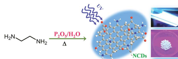
Scheme 1 Synthesis of NCDs by carbonization of ethylenediamine. Photographs (solution phase (top) and solid powder (bottom)) show white light emission under 365 nm UV light.
