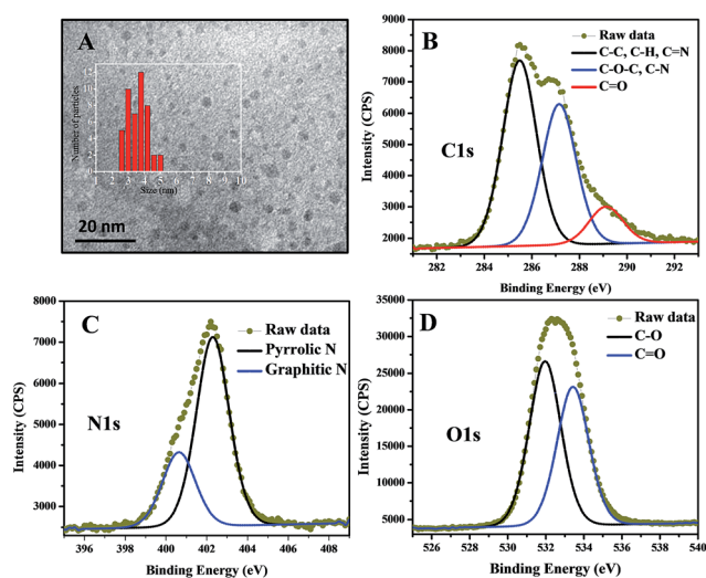
Fig. 1 (A) TEM image of prepared NCDs, inset: histogram showing the size distribution. (B–D) are the high resolution XPS spectra of C1s, N1s and O1s, respectively.
