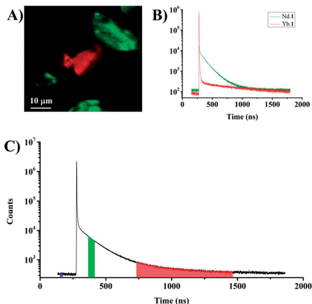
Fig. 4 (A) 100 \times 100 pixels photon arrival time image (PARTI) of silica particles dyed with either Nd.1 (green) or Yb.1 (red). Total integrations time 1000 s. (B) Time resolved emission profiles of Nd.1 (green) and Yb.1 (red) extracted from the photon stream. (C) Full time-resolved emission profile recorded by TCSPC while imaging. The red, blue, and green arrival time intervals are selected to generate the best photon arrival time resolved image.
