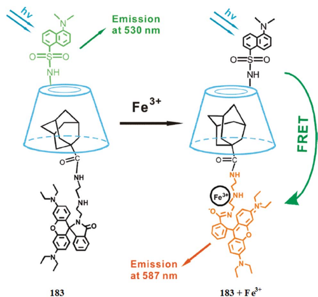
Fig. 151 Formation of the AD-SRhB/β-CD-DNS supramolecular complex 183 and its FRET-based ratiometric sensing of ferric ions in aqueous media.
