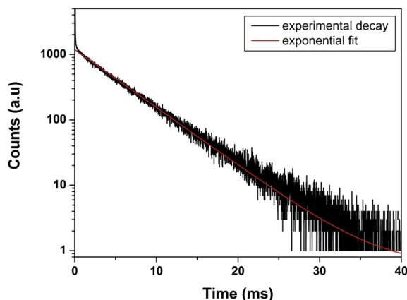
Fig. 8 Photoluminescence decay profile of \text{LaPO}_4:\text{Eu}^{3+} (0.5 mol%) at emission and excitation wavelengths of 593 and 256 nm, respectively.
