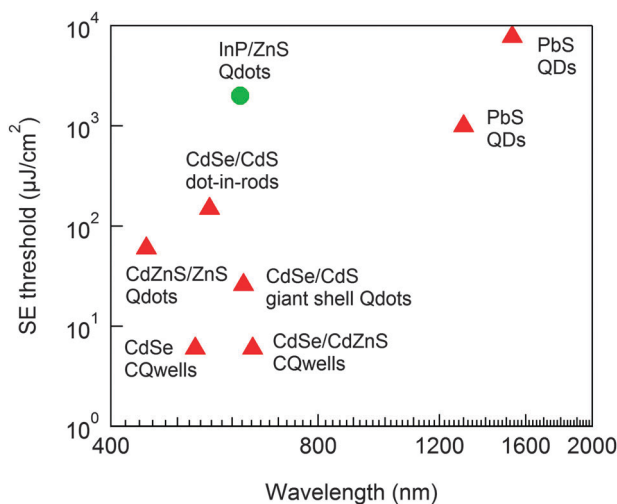
Fig. 11 Stimulated emission thresholds as a function of wavelength for InP/ZnS QDs, 213 PbS QDs (1.3 \mu\text{m} , ref. 218 and 1.52 \mu\text{m} , ref. 218), CdSe/CdS dot-in-rods, 217 CdZnS/ZnS QDs, 31 giant shell CdSe/CdS QDs, 228 CdSe/CdZnS CQwells, 225 and CdSe CQwells, 28 highlighting both the lack of heavy-metal-free and the high threshold and scarce reports of NIR NC gain media.
