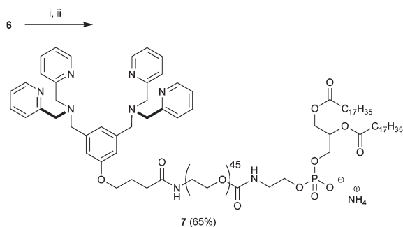
Scheme 2 Preparation of BDPA-PEG 2000 -DSPE ( 7 ). Conditions: (i) PfpOH, EDC, DMAP, \text{CHCl}_3 , 0 °C to rt, 16 h followed by (ii) \text{H}_2\text{N-PEG}_{2000}\text{-DSPE} , DIPEA, \text{CHCl}_3 , rt, 24 h.
