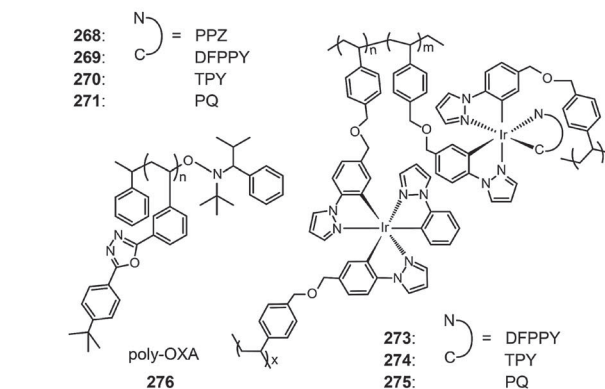
Fig. 18 procedure of solution-processed multi-layer devices on the basis of crosslinkable monomers 268–271 and the corresponding crosslinked polymers 272–275. (Reproduced with permission from ref. 116. Copyright 2009, Wiley-VCH Verlag GmbH & Co. KGaA.)
