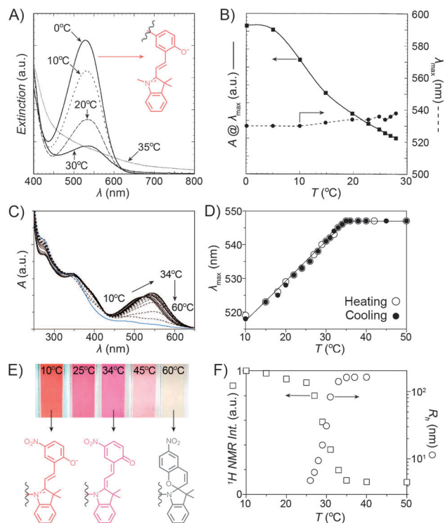
Fig. 9 Spiropyran as a probe for microenvironment polarity. (A) Thermally induced MCH + → SP transition (0–30 °C) precedes precipitation of poly(NIPAM-SP) (35 °C). (B) Changes in maximum absorbance values and wavelength absorption maxima at temperatures below the volume phase transition. (C) Optical response of a poly(NIPAM-SP) polymer pre-irradiated with UV as it is gradually heated from T = 10^\circ\text{C} to T = 60^\circ\text{C} . (D) Temperature-dependent changes in wavelength absorption maxima of the same copolymer. (E) Colour changes accompanying a gradual zwitterion → quinoid conversion (observed spectrophotometrically in (C)). (F) Precipitous drop of the integrated intensity of the NIPAM's CH proton resonances (left) coincides with the rapid increase of the hydrodynamic radius (right). [Adapted with permission from ref. 223 (Copyright 2004 American Chemical Society) (A and B) and ref. 224 (Copyright 2009 American Chemical Society) (C–F).]
