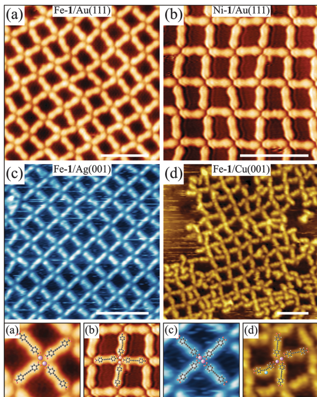
Fig. 1 (a) Fe- 1 and (b) Ni- 1 fully reticulated network structures on Au(111) (metal atom : 1 ratio 1 : 1). The same Fe- 1 networks can also be obtained on (c) Ag(001) and (d) Cu(001) substrates. Models for each structure are shown in the corresponding bottom panels. Structures were obtained by simultaneous deposition of metal atoms and 1 at 450 K on the substrates. Images acquired at 5 K (a, b) and 300 K (c, d). Scale bars are 5 nm.
