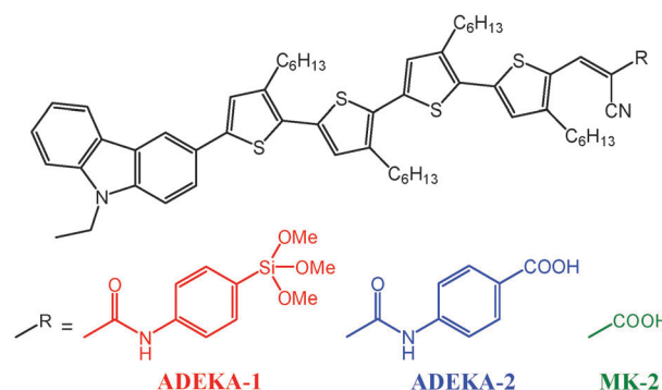
Fig. 1 Molecular structures of carbazole dyes with a trimethoxysilyl group (ADEKA-1) and with a carboxy group (ADEKA-2 and MK-2) as the anchor moiety for chemical bonding to the surface of the \text{TiO}_2 electrodes.
