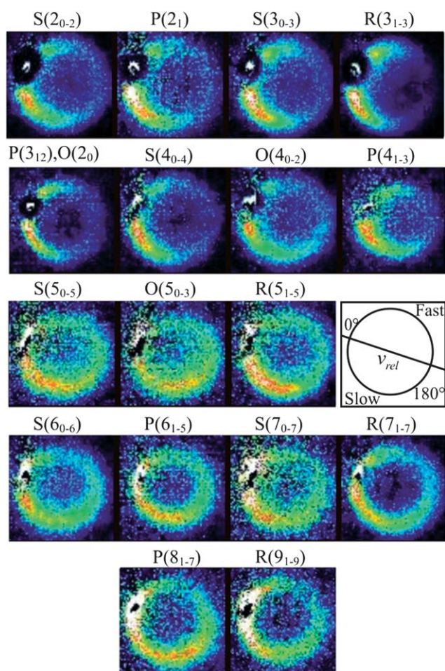
Fig. 4 Raw images for inelastic scattering of \text{CD}_3 radicals by He at a collision energy of 440 \pm 35 \text{ cm}^{-1} . The images are denoted by the symbol Y(n'_{k'-k''}) for final rotational levels from n' = 2-9 , with unresolved final k' projection levels as discussed in the text. Y denotes the spectroscopic branch. The rotational angular momentum of the incident \text{CD}_3 beam was predominantly n = 1 (see Table 1 for the complete incident level distribution). The orientation of the relative velocity vector v_{\text{rel}} is indicated in one panel.
