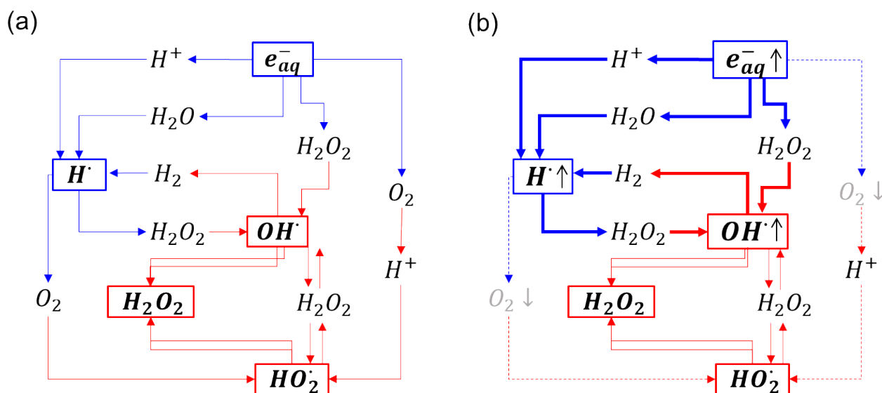
Figure 1. A schematic diagram of interconversion between reactive species during water radiolysis by e-beam irradiation (modified from Ponomarev and Ershov 23 ) under (a) oxidic and (b) suboxic/anoxic conditions. Blue and red lines represent the pathways involving reducing and oxidizing reactive species, respectively. Bold and dashed lines indicate potentially enhanced and declined reactions, respectively, at low DO conditions.
