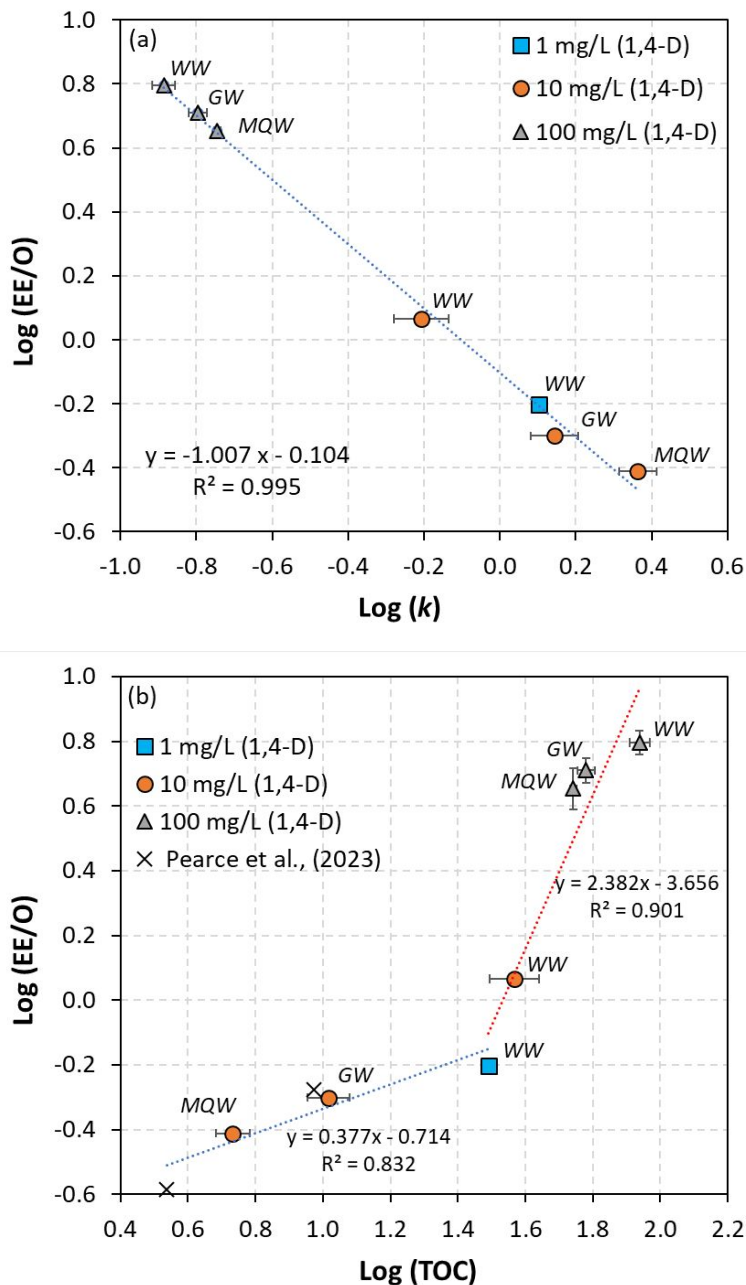
Figure 5. Relationship (Log-Log) between calculated EE/O values ( \text{kWh/m}^3/\text{order} ) and (a) pseudo-first-order reaction rate constants ( 1/\text{kGy} ) and (b) TOC concentrations. Marker shape represents different targeted initial 1,4-dioxane concentrations (1 to 100 mg/L) and the type of water matrix (MQW, GW, and WW) is denoted next to each data point. The background TOC value in GW and WW was \sim 5.1 mg-C/L and \sim 31 mg-C/L, respectively. Two data points (cross) are acquired from Pearce et al. 33 in panel (b).
