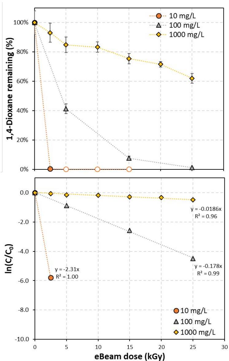
Figure 2. Degradation of 1,4-dioxane as a function of the e-beam dose. Error bars represent the standard error of two replicate measurements. The open circle indicates below the detection limit. Average measured initial concentration: [C_0, 10 \text{ mg/L}] = 9.81 \text{ mg/L} , [C_0, 100 \text{ mg/L}] = 100.7 \text{ mg/L} , and [C_0, 1000 \text{ mg/L}] = 1029 \text{ mg/L}
