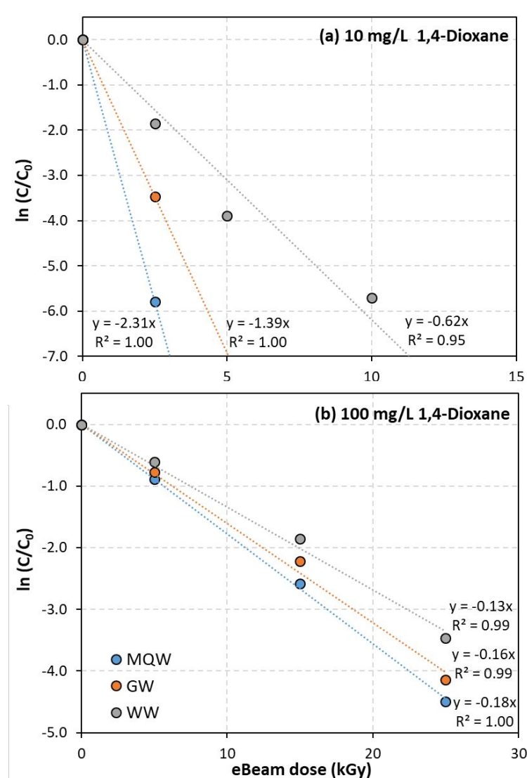
Figure 4. Degradation kinetics with the initial 1,4-dioxane concentration of (a) 10 mg/L and (b) 100 mg/L in pure water (MQW), contaminated groundwater (GW), and wastewater (WW). Average measured initial 1,4-dioxane concentration: [C_0, 10 \text{ mg/L MQW}] = 9.81 \text{ mg/L} , [C_0, 10 \text{ mg/L GW}] = 10.1 \text{ mg/L} , [C_0, 10 \text{ mg/L WW}] = 10.0 \text{ mg/L} , [C_0, 100 \text{ mg/L MQW}] = 100.7 \text{ mg/L} , [C_0, 100 \text{ mg/L GW}] = 96.1 \text{ mg/L} , [C_0, 100 \text{ mg/L WW}] = 102.9 \text{ mg/L}
