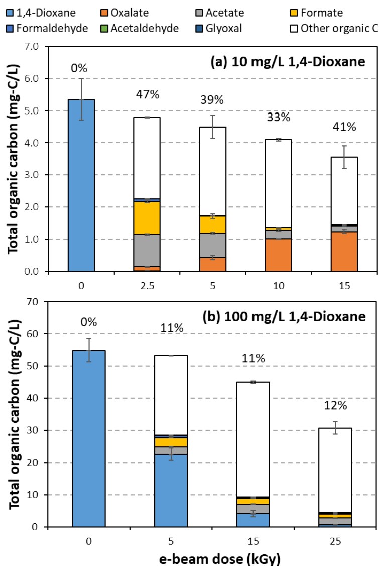
Figure 3. Byproduct formation as a function of e-beam dose at two initial 1,4-dioxane concentrations: (a) 10 mg/L ( \sim 5.45 mg-C/L) and (b) 100 mg/L ( \sim 54.5 mg-C/L); [Other organic carbon] = [total organic carbon] – \sum [measured byproducts]. The value above each bar represents the percentage of measured byproducts (in C mass) out of total organic carbon.
