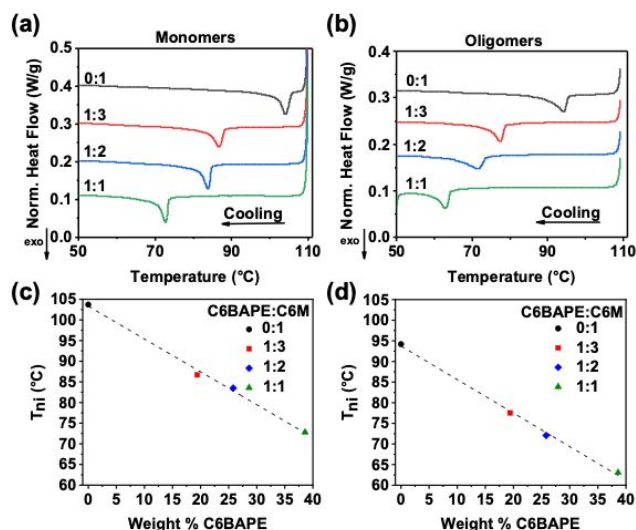
Fig. 2 DSC thermograms of (a) monomer mixtures and (b) oligomers used to prepare monodomain azobenzene-functionalized LCE. The T_{ni} of these materials is plotted as a function of C6BAPE concentration for (c) monomer mixtures and (d) oligomers.
