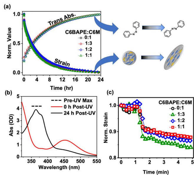
Fig. 5 (a) Normalized photoinduced strain relaxations (solid symbols) for monodomain azobenzene-functionalized LCE films monitored for 24 h in the dark following 365 nm light exposure (20 min, 50 mW/cm 2 ) and normalized trans absorbance (open symbols) of azobenzene-functionalized films monitored for 24 h in the dark following 365 nm light exposure (20 min, 50 mW/cm 2 ) to show cis-trans thermal relaxation. (b) Representative (1:3 composition) UV-Vis spectra collected at 0 h and 24 h after removal of UV light. (c) First five minutes of photoinduced strain relaxation experiments with removal of UV light occurring at 1 min.
