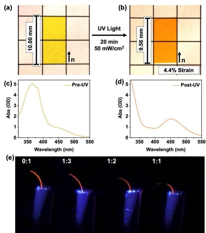
Fig. 6 Images of azobenzene-functionalized LCE (1:2 composition) (a) before and (b) after UV light exposure (365 nm, 20 min, 50 mW/cm 2 ). UV-Vis spectra for film (c) before and (d) after UV exposure. (e) Monodomain azobenzene-functionalized LCE cantilevers (.005 mm x 1 mm x 6 mm, increasing C6BAPE concentration from left to right) after 2 seconds of 365 nm light exposure (50 mW/cm 2 )
