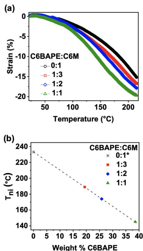
Fig. 3 (a) Thermomechanical strain generated by azobenzene-functionalized LCE (0.001 N constant force) as temperature was ramped at 3°C/min (b) T_{ni} calculated by inflection point of thermomechanical strain curves and plotted as a function of C6BAPE concentration. Composition 0:1 did not reach an inflection point before degradation, so T_{ni} was extrapolated by linear fit of T_{ni} plotted against C6BAPE concentration for the other three compositions and plotted as 0:1.
