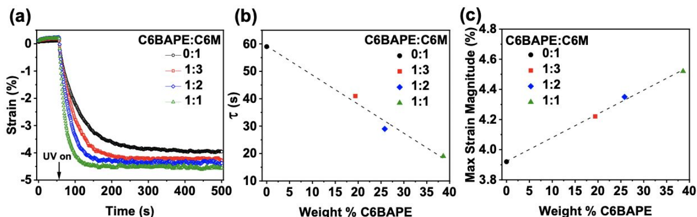
Fig. 4 (a) Photomechanical strain generated by azobenzene-functionalized LCE. (0.001 N constant force, 50 mW/cm 2 , 365 nm light exposure at 60 s) (b) Time constants as a function of C6BAPE concentration calculated from exponential fitting of photomechanical strain curve. (c) Maximum photomechanical strain as a function of C6BAPE concentration.
