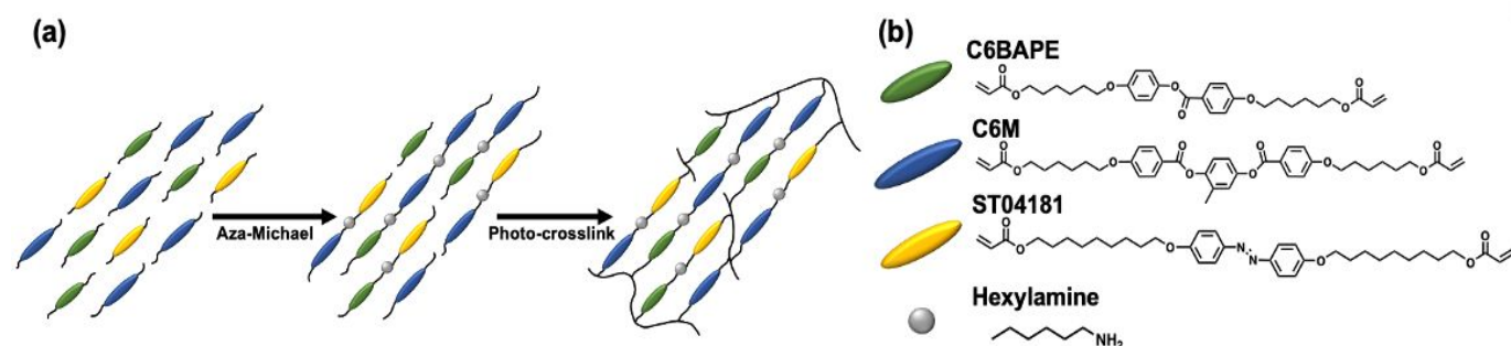
Fig. 1. (a) Generalized synthetic approach to prepare azobenzene-functionalized liquid crystalline elastomers (azo-LCE) by a one-pot, two-step polymerization method utilizing aza-Michael addition and subsequent photopolymerization. (b) The liquid crystalline monomers C6BAPE, C6M, and ST04181 were mixed with hexylamine to prepare monodomain azobenzene-functionalized LCE
