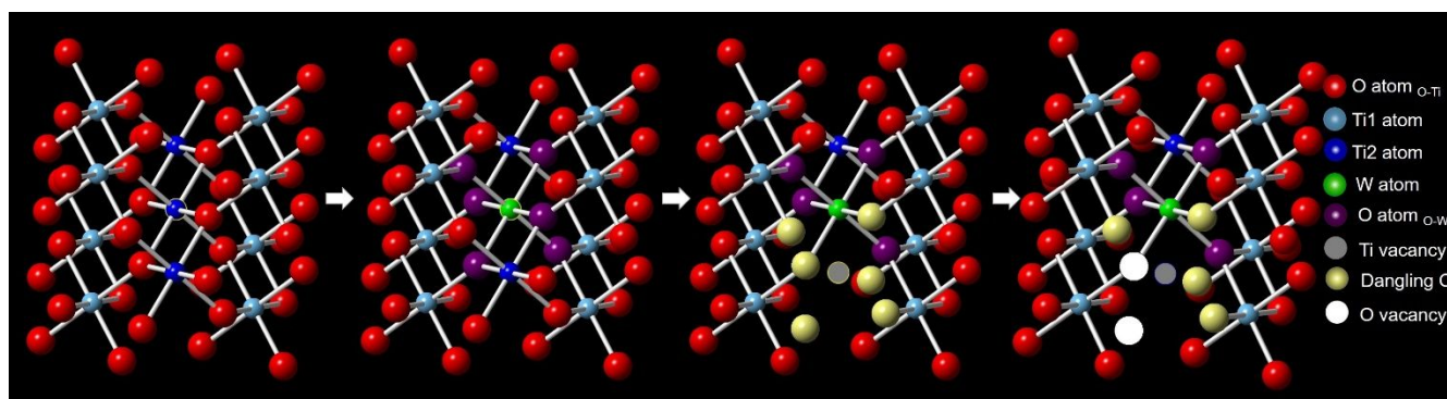
Figure 7. A schematic illustration of W-doping induced structural change to \text{TiO}_2 .
