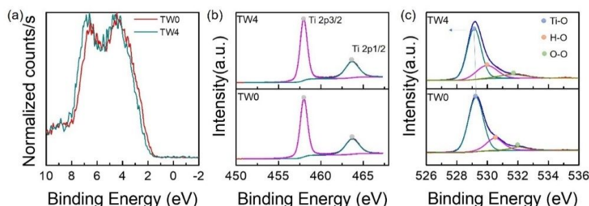
Figure 4. (a) Valence band and XPS spectra of (b) Ti 2p and (c) O 1s core level of the as-prepared samples.
