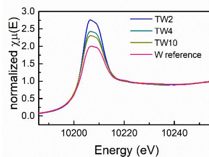
Figure 5. W L_3 -edge XANES spectra of three W-doped \text{TiO}_2 and W-reference samples.
