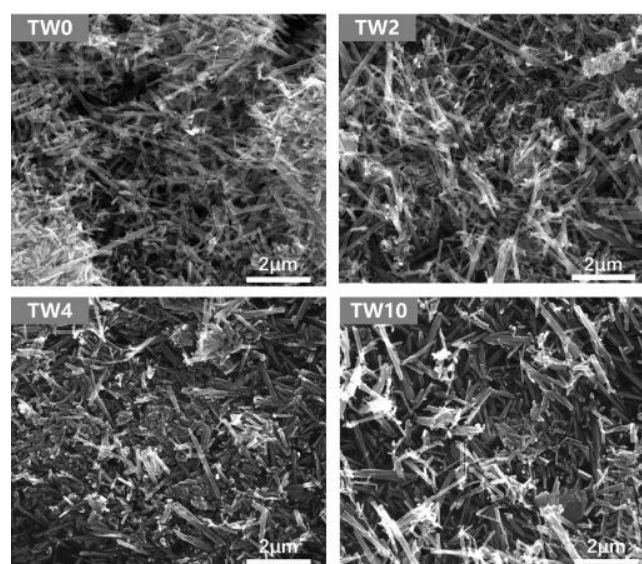
Figure 1. SEM images of TW0, TW2, TW4 and TW10.
