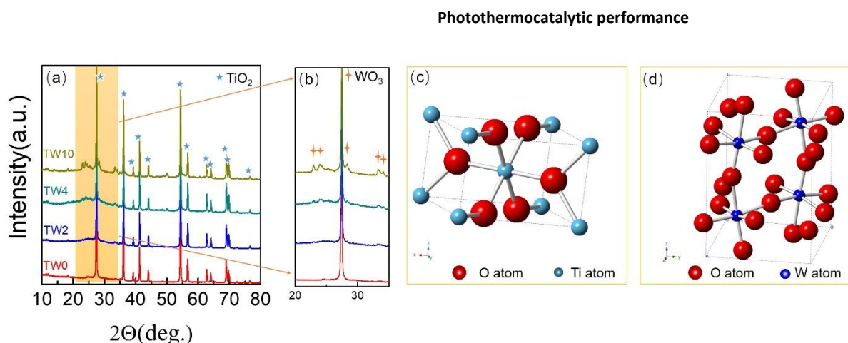
Figure 2. (a) XRD patterns and (b) magnified XRD patterns in the region of 20-35 degrees of TW0, TW2, TW4 and TW10. (c) TiO 2 and (d) WO 3 unit cell images.
