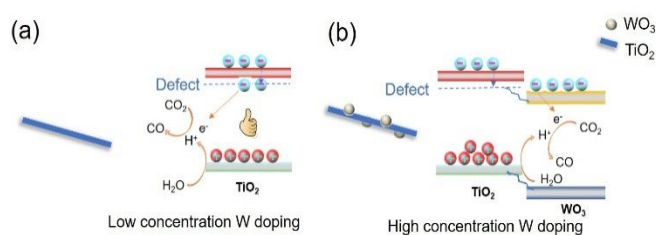
Figure 8. Scheme of W-doped \text{TiO}_2 over different doping concentration.
