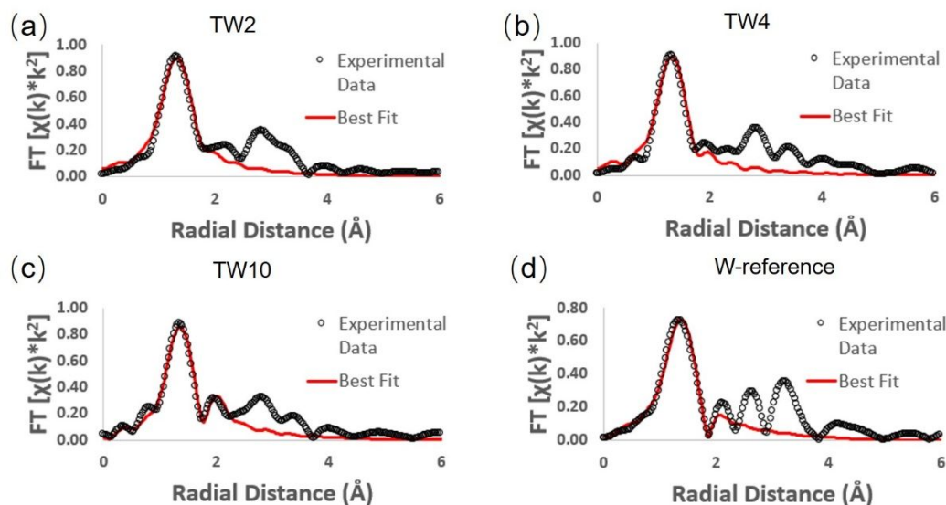
Figure 6. W L_{3} -edge FT-EXAFS spectra of different samples.
