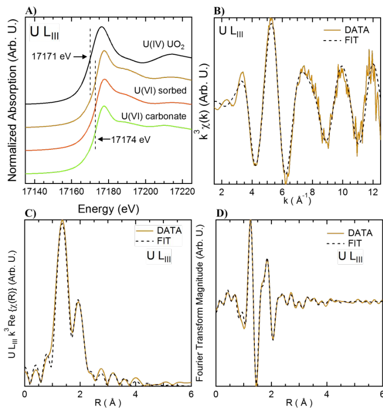
Figure 3 XAS analysis of root section incubated with 100 \mu\text{M} U. Orange line is the sample spectra. Panel A: U L III XANES spectra; Panel B: k 3 U L III EXAFS fitting; Panel C: shell fitting of the U L III EXAFS spectra; Panel D: Fourier Transform fitting. Dashed lines represent the fitted data.
