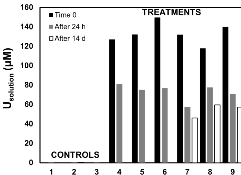
Figure 2 Uranium concentration in solution in the in vitro experiments for controls (samples 1-3) containing 0 \mu\text{M} U, and replicates (samples 4-9) containing 100 \mu\text{M} U. Samples were collected at time zero (full bars), after 24 h of incubation (grey bars), and after 14 d of incubation in controls 1 and 2, and samples 7, 8, and 9 (empty bars).
