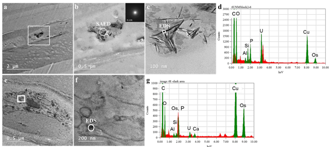
Figure 5 High resolution TEM of the root section incubated with 100 μM U for 24 h with Electron Dispersive Analysis (EDS). Images in the top row shows a plant root cell with a high-density material in the region inside the square (panel a), with energy diffraction pattern of particles in A in panel b, EDS of the particles in the panel c shown in panel d. The bottom row show a different conglomerate of cells in panel e, and the EDS of the particles in panel f shown in panel g.
