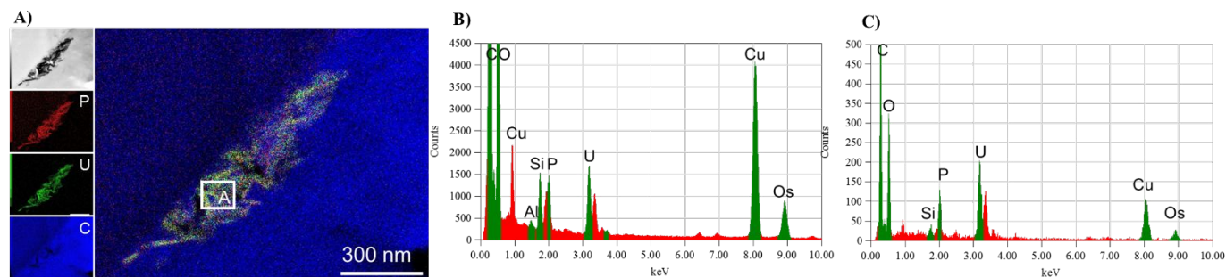
Figure 6 TEM-EDS mapping of a particle agglomerate (panel A) inside with cumulative EDS of the whole area and the EDS from section A in the map.
