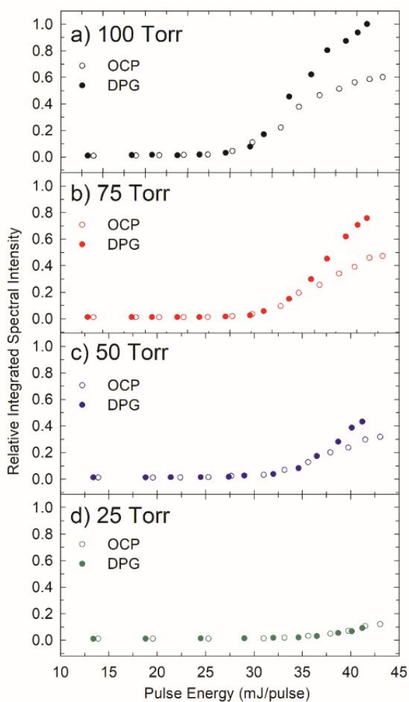
Figure 4. Relative integrated spectral intensities at pressures of a) 100 Torr, b) 75 Torr, c) 50 Torr, and d) 25 Torr with either the optical centrifuge polarization (OCP) or dynamic polarization grating (DPG) polarizations.
