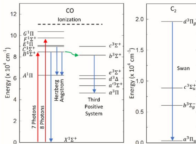
Figure 7. Electronic energy levels and terms for CO and C 2 . The red arrows indicate multiphoton absorption of seven and eight 800 nm photons. Emission is indicated with blue arrows and collision-induced intersystem crossing (denoted in green) leads to excitation of CO triplet states.
