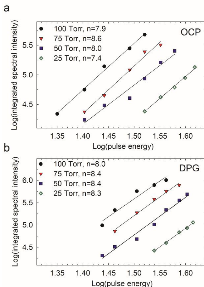
Figure 6. Power-dependent analysis to determine the lower limit for the number of photons absorbed by CO that initiate formation of C_2(d^3\Pi_g) . Log-log plots of integrated spectral intensity vs pulse energy for (a) the optical centrifuge polarization and (b) the dynamic polarization grating.
