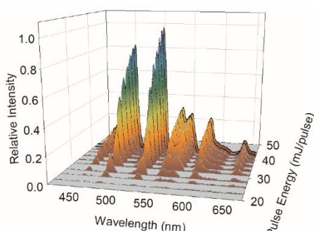
Figure 3. Power-dependent Swan Band emission spectra with cell pressure of 100 Torr and optical centrifuge polarization.
