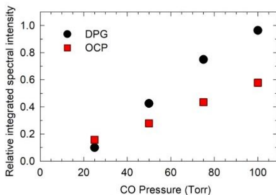
Figure 5. Comparison of relative integrated C_2 emission intensity for optical centrifuge polarization (OCP) and the dynamic polarization grating (DPG) as a function of cell pressure with I = 1.8 \times 10^{13} \text{ W cm}^{-2} (41 mJ/pulse).
