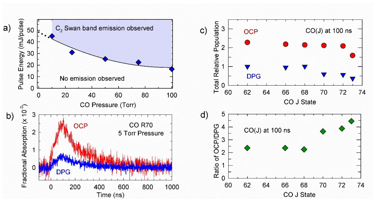
Figure 8. a) The pressure dependence of the Swan band emission threshold. b) R-branch high-resolution transient IR absorption for the CO J=70 state with OCP and DPG excitation. c) J -dependent transient intensities at 100 ns based on polarization-sensitive IR detection. d) Ratio of S(J) values with OCP and DPG.
