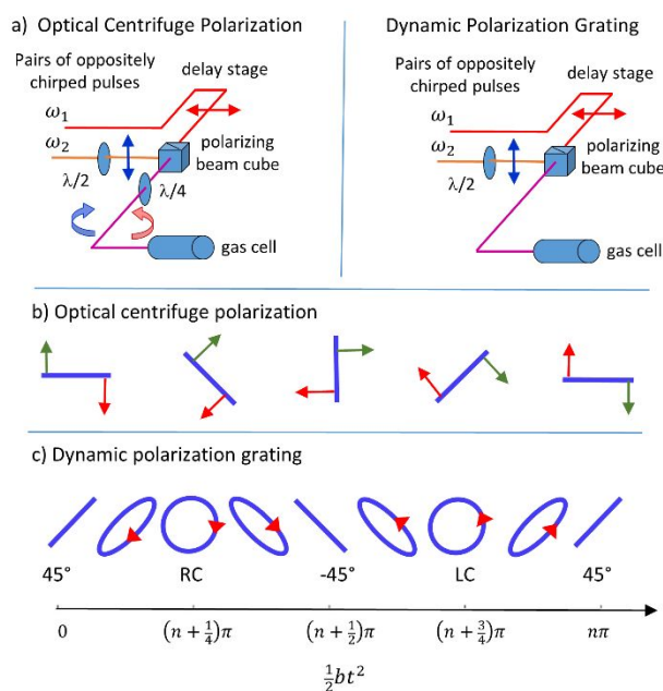
Figure 2. a) Experimental setup for generating light with optical centrifuge polarization and a dynamic polarization grating. b) The optical centrifuge has linearly polarized light that angularly accelerates over the time of the pulse. c) The dynamic polarization grating changes polarization from 45^\circ linear, to right circular, to -45^\circ linear, to left circular and back to 45^\circ linear.
