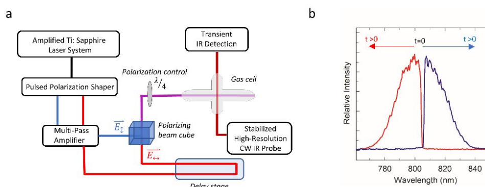
Figure 1. a) Schematic of experimental set up. An amplified Ti: sapphire laser system is spectrally divided into two pulses in a polarization shaper. The two pulses are then amplified with a multi-pass amplifier and combined with a polarizing beam cube. Stabilized high-resolution CW IR probe is used to measure transient population of specific rotational states. b) Spectral output of the polarization shaper.
