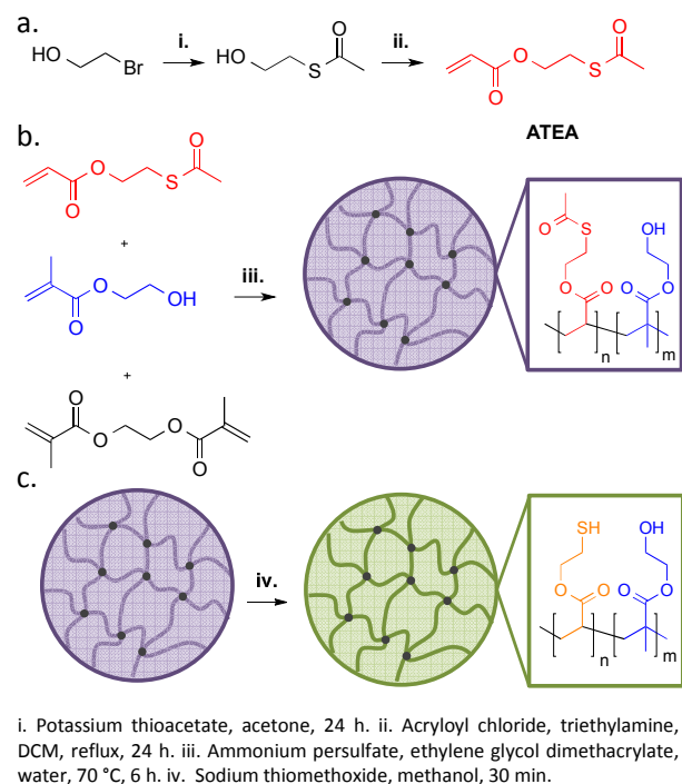
Fig. 1a. Synthetic route to ATEA, a protected thiomonomer. b. polymerisation to form ATEA:HEMA copolymer microgels, displaying the pendant functionalities present. c. deprotection of ATEA using sodium thiomethoxide to yield thiol-bearing microgels.
