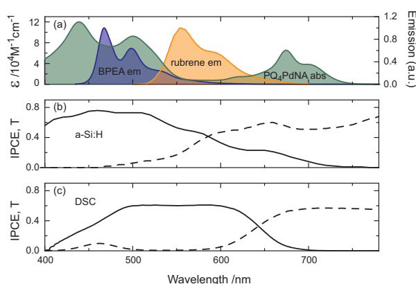
Fig. 3 The spectral properties of the two UC/device assemblies in this study: (a) absorption of \text{PQ}_4\text{PdNA} (green) and emission of rubrene (orange) and BPEA (blue). IPCE (solid) and transmittance (dash) of (b) a-Si:H, illuminated through glass substrate and (c) DSC, illuminated through working-electrode.
