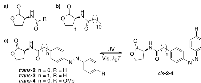
Figure 1. Molecular structures of AHLs. a) The structure of naturally-occurring AHLs, where R is usually an alkyl chain varying in length between 4 and 18 carbon atoms. b) Structure of a naturally occurring auto-inducer (1) c) Three photoswitchable analogs (2, 3 and 4) that can undergo trans-cis photoisomerization upon UV-light irradiation and cis-trans isomerization upon visible-light irradiation and thermal relaxation.
