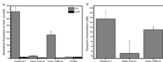
Figure 3 Gene expression and pyocyanin production in P. aeruginosa . a) Effect of compounds 1 (10 \mu M) and 3 (100 \mu M) on the gene expression of las -controlled genes in P. aeruginosa . Gene expression of lasA in the presence of non-irradiated compound 3 , 365 nm irradiated 3 and compound 1 in the \Delta lasI (gray) and \Delta lasRI (black) strains. All samples are compared to the control sample. Data is plotted as mean and standard deviation of two biological replicates each performed in duplo. b) The effect of compounds 1 (50 \mu M) and 3 (2x50 \mu M) on pyocyanin production in cultures of P. aeruginosa \square lasI before and after \lambda=365 nm light-irradiation. Data is plotted as mean and standard deviation of three experiments consisting of two biological replicates.
