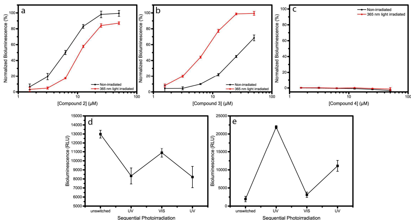
Figure 2 Dose-response curves of compounds 2 , 3 and 4 , before and after irradiation, obtained by measuring the Las QS controlled bioluminescence at different concentrations, using the E. coli JM109 pSB1075 sensor strain. Dose-response curve of non-irradiated (black) and \lambda=365 nm light-irradiated (red) compounds 2 (a), 3 (b) and 4 (c). d) and e) Effect of photoswitching on the biological activity of compounds 2 (d) and 3 (e). Both compounds were used at a concentration of 6.25 \mu\text{M} for the sequential rounds of photoirradiation. Data points and error bars represent the mean and pooled standard deviation of two biological replicates each performed in triplicate.
