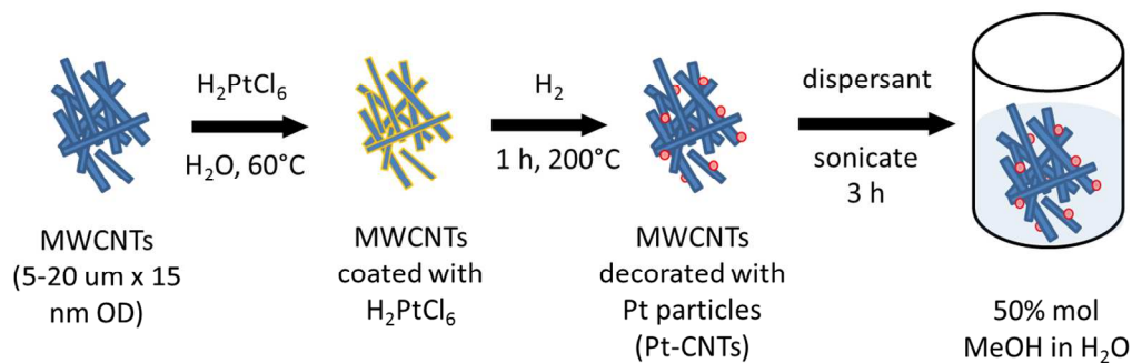
Scheme 1. Synthetic approach for Pt decorated carbon nanotubes (Pt-CNTs).
