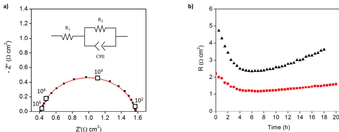
Figure 7. Symmetric cell impedance measurements Pt-CNT based electrodes prepared by strategy 2: a) Nyquist plot for 46 wt% Pt-CNT-CsH 2 PO 4 composite after 4 hours (inset: equivalent circuit used for fitting) and b) temporal evolution of the electrode resistance values of 30 wt% (black) and 46 wt% (red) Pt-CNT-CsH 2 PO 4 composites, showing higher stability in the electrolyte with higher Pt loading.
