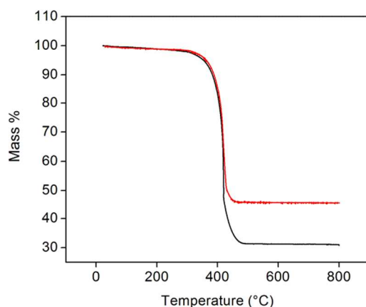
Figure 3. TGA profiles of 30 (black) and 46 wt% (red) Pt-CNTs (measured under flowing air at a heating rate of 2 °C \text{min}^{-1} ).
