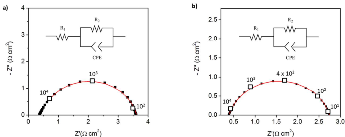
Figure 6. Symmetric cell impedance measurements of 30 wt% Pt-CNT based electrodes prepared by (a) strategy 1 (see Scheme 2) in which Pt-CNT bearing and CDP bearing solutions were electrospayed sequentially, and (b) strategy 2 in which a single Pt-CNT and CDP bearing solution was sprayed. In (a), the Pt loading and utilization are 4.6 \times 10^{-3} \text{ mg cm}^{-2} Pt and 65 \text{ S mg}^{-1} , respectively, whereas in (b) they are 5.1 \times 10^{-3} \text{ mg cm}^{-2} Pt and 85 \text{ S mg}^{-1} . Measurements are performed at 240 \text{ }^\circ\text{C} in a dynamic atmosphere of 0.4 \text{ atm H}_2\text{O} and balance \text{H}_2 supplied at a gas velocity of 6 \text{ cm min}^{-1} and spectra are taken after 4 hours (insets: equivalent circuit used for fitting).
