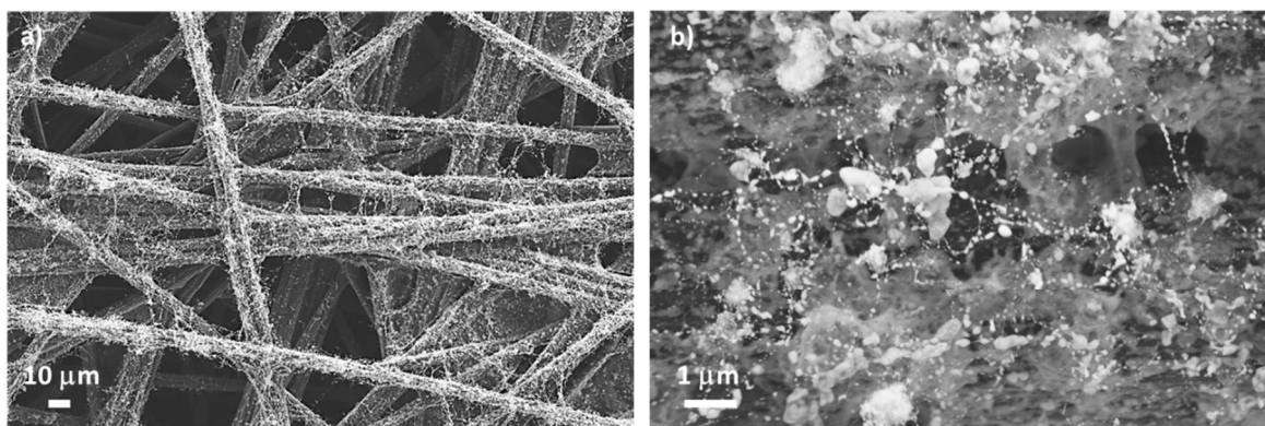
Figure 5. SEM images of electrospayed 46 wt% Pt-CNT- \text{CsH}_2\text{PO}_4 composites, showing direct contact between the electrolyte particles with the carbon nanotubes: (a) low and (b) high magnification.
