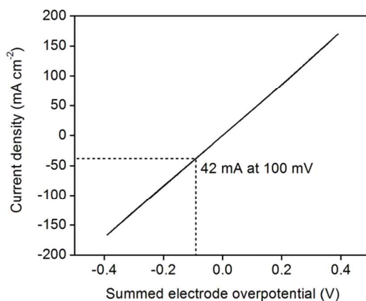
Figure 8. IR-corrected polarization curve of a 46 wt% Pt-CNT-CsH 2 PO 4 composite electrode at 1 mV s -1 , showing high current density at low overpotentials for both proton reduction and hydrogen oxidation.
