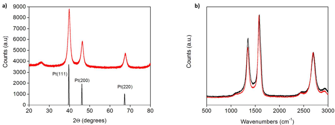
Figure 1. a) X-ray powder diffraction of 46 wt% Pt-CNTs (red) along with a reference trace 25 (black), and b) Raman spectra of as-received (red) and 46 wt% Pt-decorated (black) commercial CNTs showing that the carbon nanotube structure is largely unchanged after decoration.
