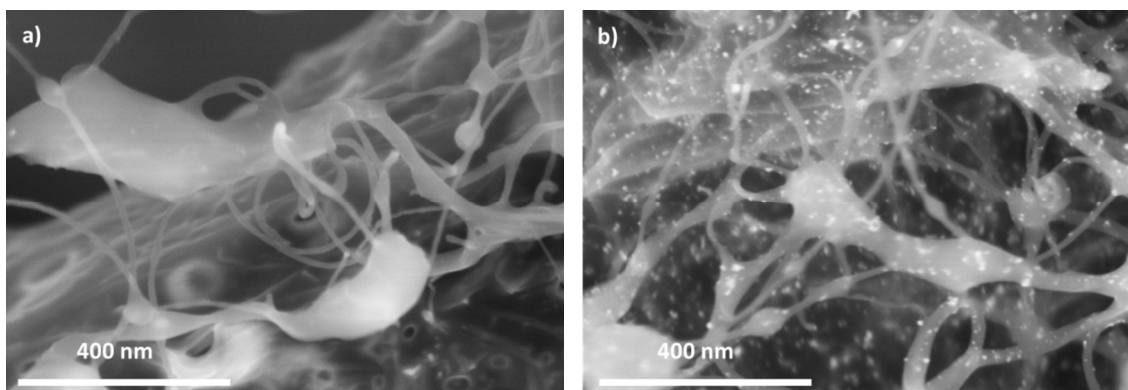
Figure 2. High resolution SEM images of (a) as received and (b) 46 wt% Pt-decorated commercial CNTs. Pt nanoparticles with diameters of < 17 nm are evident in the latter. Bundling and agglomeration of CNTs is evident in both images.
