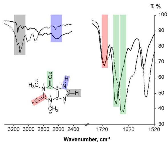
Figure 11. FTIR spectra of theophylline Form II (—) and Form IV (---), showing carbonyl group, alkene group hydrogen bond and imidazolium group hydrogen bond stretching band assignment.
