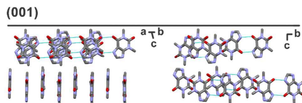
Figure 5. Crystal packing in theophylline Form IV along (001) plane. Hydrogens are omitted for clarity.
