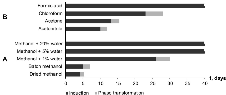
Figure 8. Induction and phase transformation times of SMPT from theophylline Form II to Form IV at 23 °C depending on used solvent environment. No phase transformation to Form IV was been observed in formic acid and methanol/water mixtures with 5% and 20% of water within the studied period (40 days).
