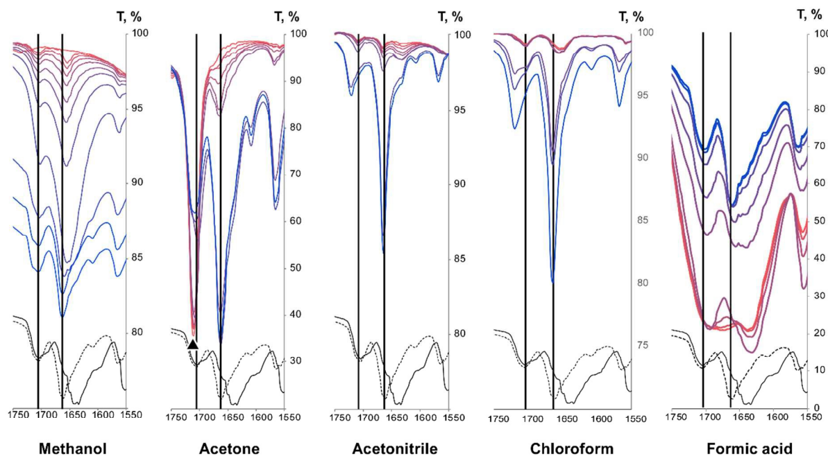
Figure 12. FTIR spectra of carbonyl group stretching band region during theophylline crystallization from saturated solutions upon solvent evaporation at room temperature. Colour gradient shows FTIR spectra changes throughout crystallization (red – saturated solution, blue – crystallization product). FTIR spectra of solid theophylline Form II (dashed line) and IV (continuous line) are added for comparison purpose. Acetone carbonyl group stretching band is marked with \blacktriangle .
