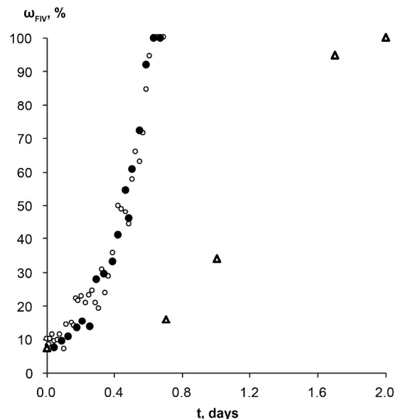
Figure 7. Weight fraction of the theophylline Form IV in the SMPT from theophylline Form II/Form IV mixture ( w_{II}/w_{IV} ; 90/10) to Form IV, in saturated (o) Form IV and (●) Form II methanol solutions at 23 °C. \Delta represents the weight fraction of the theophylline Form IV in the solid phase during the SMPT from theophylline Form II in methanol at 23 °C. All kinetic curves are aligned to the point when solid phase of respective SMPT contained 10% of Form IV.
