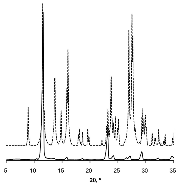
Figure 4. PXRD patterns of Form IV obtained by SMPT in methanol (—); and simulated from crystal structure (---).
