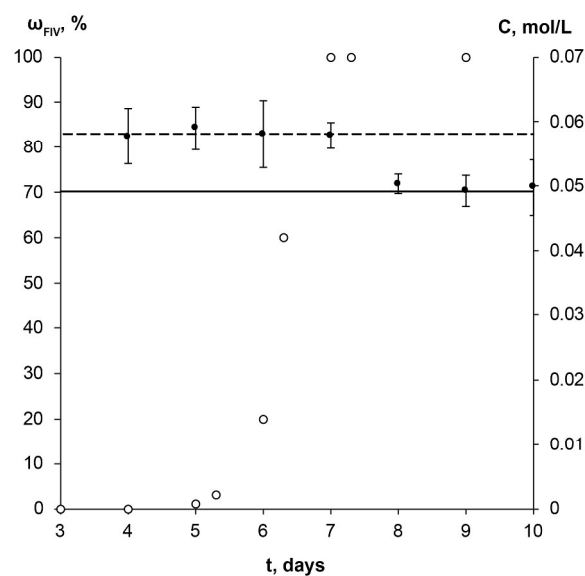
Figure 2. Solution concentration (●), and weight fraction of theophylline Form IV in the solid phase (○) during the solution mediated transformation from theophylline Form II to Form IV in methanol at 23 °C. The dashed line (---)
