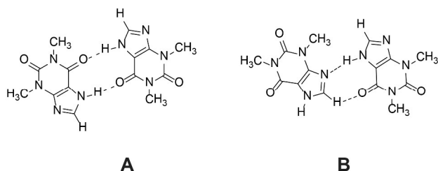
Figure 10. Theophylline dimer present in crystal structures of monohydrate, Form IV and most cocrystals (A); and the preferred theophylline dimer according to Etters rules (B).
