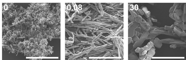
Figure 6. SEM images throughout lyophilized theophylline slurry in methanol at 23 °C. Inset: time of sample gathering (days) and 20 µm scale bar.
