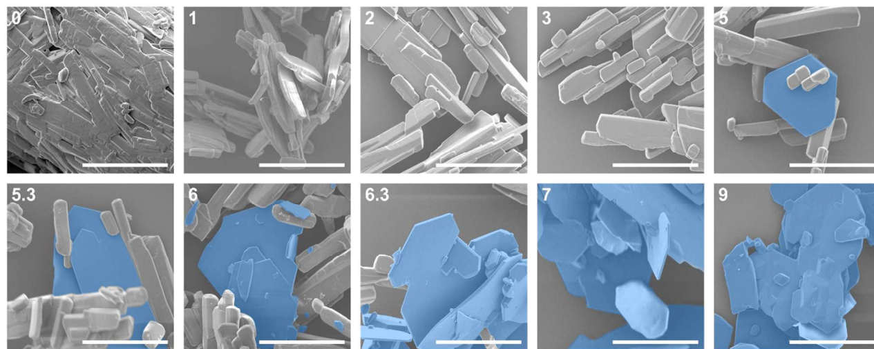
Figure 3. SEM images throughout SMPT from theophylline Form II to Form IV in methanol at 23 °C. Inset: time of sample gathering (days); 40 μm scale bar, crystals of theophylline Form IV indicated with blue colour.
