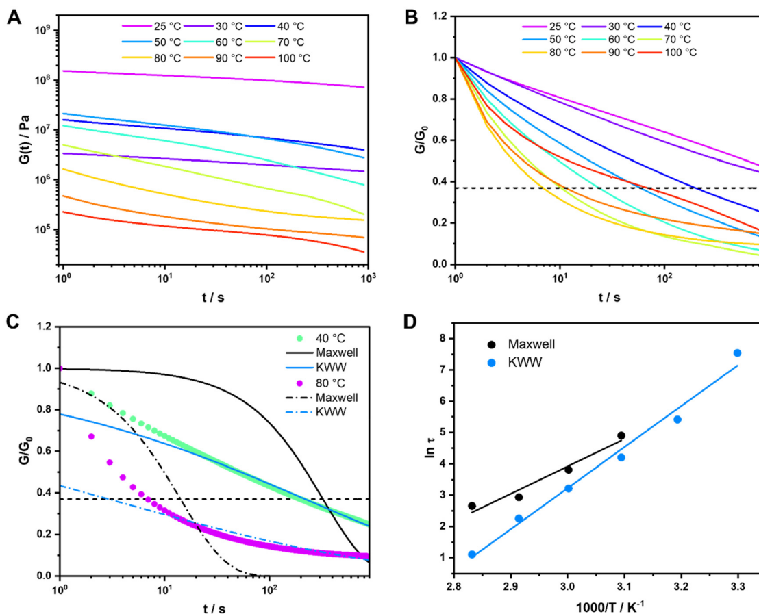
Fig. 2 Stress relaxation plots for P2-Zn : (A) stress relaxation measurement from 25 to 100 °C, (B) normalized stress relaxation plot, (C) normalized plot of the stress relaxation measurements at 40 and 80 °C fitted using the Maxwell and KWW models and (D) Arrhenius plot for Maxwell and KWW models.
