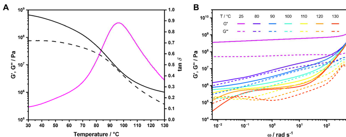
Fig. 1 Rheological plots for P2-Zn : (A) DMTA measurement from 25 to 130 °C with the storage modulus G' (black solid), the loss modulus G'' (black dotted) and the loss factor \tan \delta (violet), (B) frequency sweep from 0.00628 to 628 rad per s at different temperatures with storage modulus G' (solid lines) and loss modulus G'' (dotted lines).
