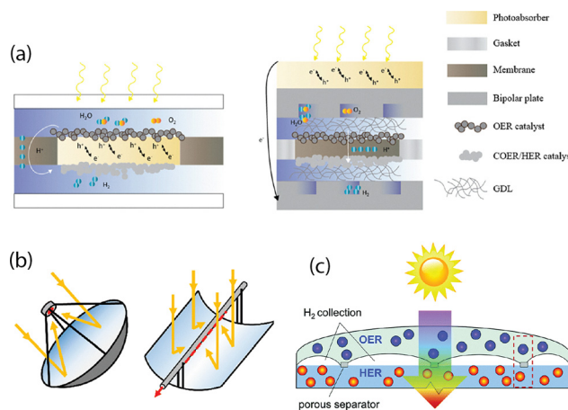
Fig. 3 Types of photoelectrochemical water splitting devices or systems that do not co-generate \text{O}_2 and \text{H}_2 , so are intrinsically safe. (a) integrated PEC systems with liquid electrolyte (left) and gas diffusion electrodes in a PV-E configuration (right), adapted with permission from ref. 17, copyright 2024, The Authors; (b) solar concentrators for PEC systems, adapted with permission from ref. 18, copyright 2024, The Authors; (c) photocatalytic particle system with redox mediator connecting the vessels, Adapted from ref. 14, with permission from the Royal Society of Chemistry.
