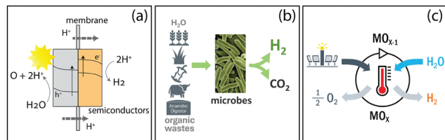
Fig. 2 Schematic of three advanced pathways. (a) photoelectrochemical (PEC); (b) biological ( \text{BioH}_2 ); (c) thermochemical (TCH) Adapted with permission from the Electrochemical Society, ref. 9, Copyright 2021. Technology details are given in the text.
