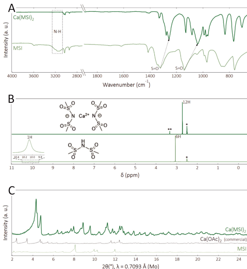
Fig. 1 (A) Infrared spectra of \text{Ca}(\text{MSI})_2 and MSI, (B) NMR spectra of MSI (*DMSO- \text{d}_6 , **water), (C) The PXRD spectra of \text{Ca}(\text{MSI})_2 , \text{Ca}(\text{OAc})_2 , and MSI.
