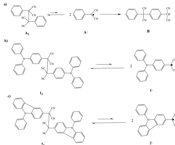
Fig. 12 (a) Equilibrium between A 2 and A • , and isomerization to B. (b) Equilibrium between I 2 and I • , (c) equilibrium between Z 2 and Z • , reproduced from ref. 45 with permission from Wiley, Angew. Chem., Int. Ed. , 2016, 55, 8634–8638, copyright 2016.
