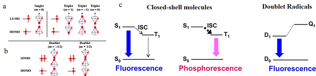
Fig. 1 Schematic diagram of the excited-state spin configurations of a closed-shell molecule (a) and a single radical (b), reproduced from ref. 1 with permission from Chinese Chemical Society, CCS Chemistry , 2020, 2, 1129–1145, copyright 2020. (c) Emission dynamics of closed-shell molecules and doublet radicals, reproduced from ref. 2 with permission from American Chemical Society, Chemical Reviews , 2024, 124, 1034–1121, copyright 2024. Note: In the excited state, HOMO and LUMO refer to the ground-state orbitals from which the electrons originate.
