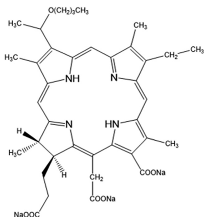
Fig. 13 Chemical structure of YLG-1.
