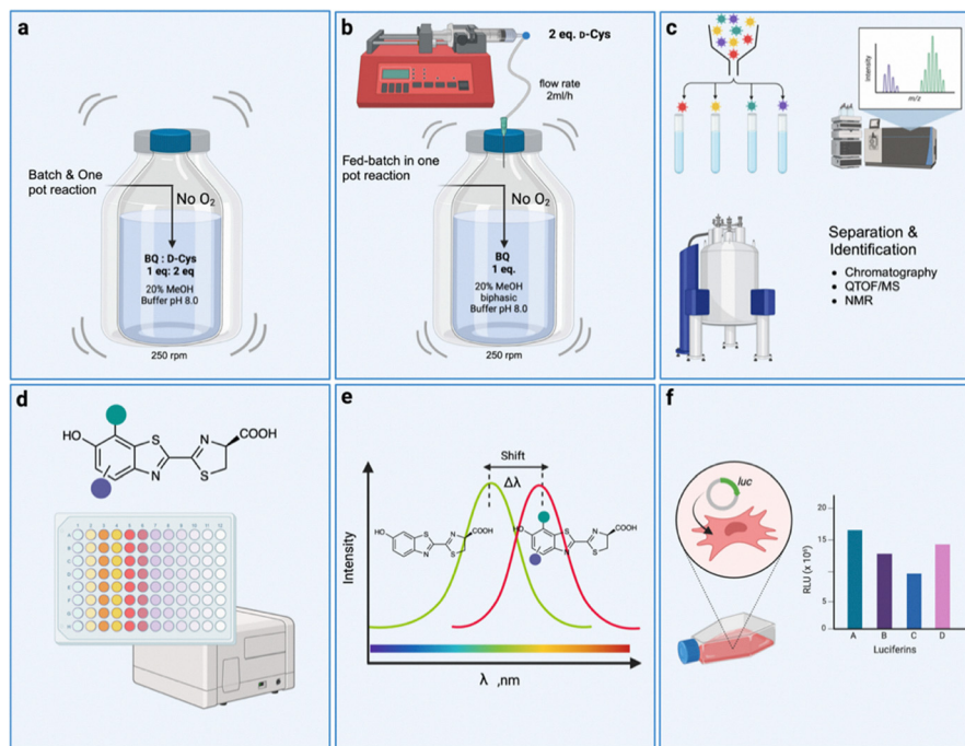
Fig. 1 Graphical representation of the overall workflow. (a) Batch and one-pot reaction for \text{D-LH}_2 synthesis. (b) Fed-batch synthesis of \text{D-LH}_2 analogues in one-pot reaction. (c) \text{D-LH}_2 analogues were isolated and characterized and their structures were elucidated by ^1\text{H} and ^{13}\text{C} NMR and high-resolution mass spectrometry. (d) BL reactions of new \text{D-LH}_2 analogues with five types of beetle luciferases. (e) BL characteristics of novel \text{D-LH}_2 analogues. (f) Demonstration of applications for new \text{D-LH}_2 analogues in mammalian cell line assays and real-time bioluminescence monitoring of live cells.
