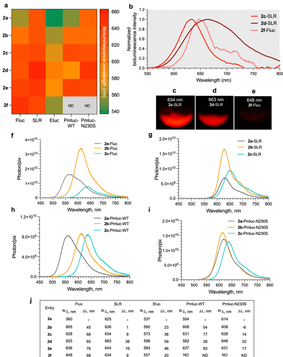
Fig. 4 BL characteristics of D -LH 2 analogues ( 2a–2f ) reacted with various luciferases. Reactions of various luciferases with D -LH 2 analogues ( 2b–2f ) were carried out at 25 °C in 100 mM HEPES buffer at pH 8.0 and compared to those of natural D -LH 2 ( 2a ). (a) Heat maps describing BL emission of D -LH 2 analogues ( 2a–2f ) generated from their reactions with Fluc, SLR, Eluc, Pmluc-WT, and Pmluc-N230S luciferases. (b) BL emission spectra of novel D -LH 2 analogues ( 2d and 2f ) obtained from their reactions with their orthogonal luciferases. (c–e) BL signals obtained from the reactions of novel D -LH 2 analogues ( 2d and 2f ) and their orthogonal luciferases were recorded by a DSLR camera. (f–i) The BL emission spectra of the luciferase (5 \mu M)–luciferin (2 \mu M) reactions were measured using the integrating sphere-based multichannel spectrometer. (j) The difference in emission wavelengths of D -LH 2 analogues ( 2b–2f ) compared to those of the natural D -LH 2 . ND denotes the non-detectable signals.
