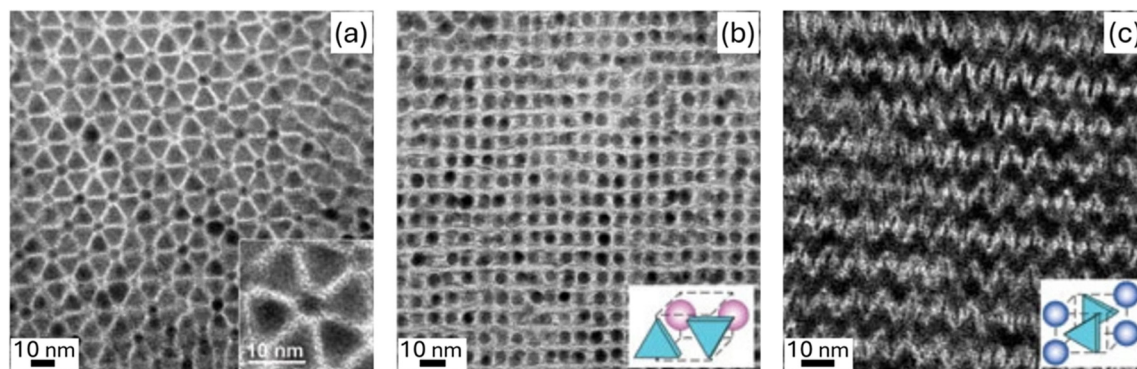
Fig. 18 TEM images of assemblies formed from \text{LaF}_3 triangular nanoplates (9.0 nm side) and 5.0 nm Au nanoparticles on (a) silicon oxide surfaces or (b) on amorphous carbon substrates. (c) TEM image of an assembly formed from \text{LaF}_3 triangular nanoplates (9.0 nm side) and 6.2 nm Au nanoparticles on amorphous carbon substrates. Insets: (a) magnified image; (b) and (c) proposed unit cells of the corresponding superstructures. Adapted with permission from ref. 31. Copyright 2006 Springer Nature.
