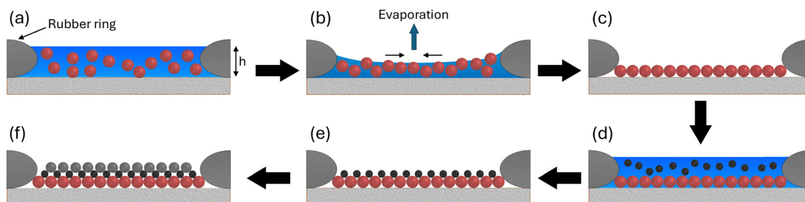
Fig. 34 Schematic illustration of the formation of ordered colloidal superstructures through confined-area evaporation-induced layer-by-layer assembly. (a) A suspension of large colloidal particles is placed inside the rubber ring. (b) As the liquid evaporates, a concave meniscus forms, creating capillary forces that bring the particles together, initiating crystal nucleation. (c) After complete evaporation, a monolayer of large colloidal particles is formed. (d) A second suspension of small particles is added inside the rubber ring. (e) Upon evaporation, the small particles settle in the gaps of the hexagonal pattern formed by the large particles, creating a binary colloidal superstructure. (f) A third suspension is added, leading to the formation of a ternary colloidal superstructure after evaporation. Adapted with permission from ref. 352. Copyright 2011 John Wiley and Sons.
