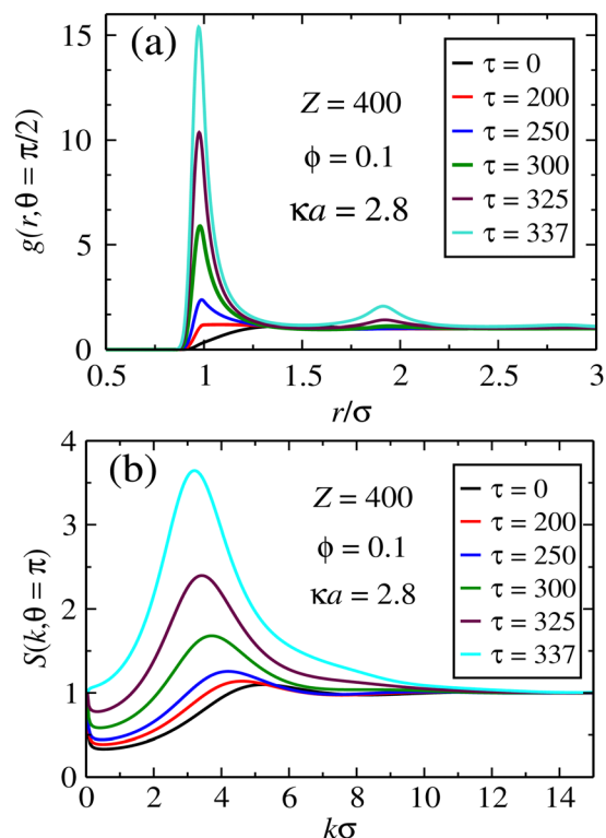
Fig. 3 Pair correlations for the case of fully screened dipoles. In (a), in-plane pair correlations indicate the formation of aggregates as \tau increases, whereas in (b) the structure factors in the transversal direction suggests a 1D crystal ordering, where the in-plane aggregates stay larger apart as \tau becomes larger.
