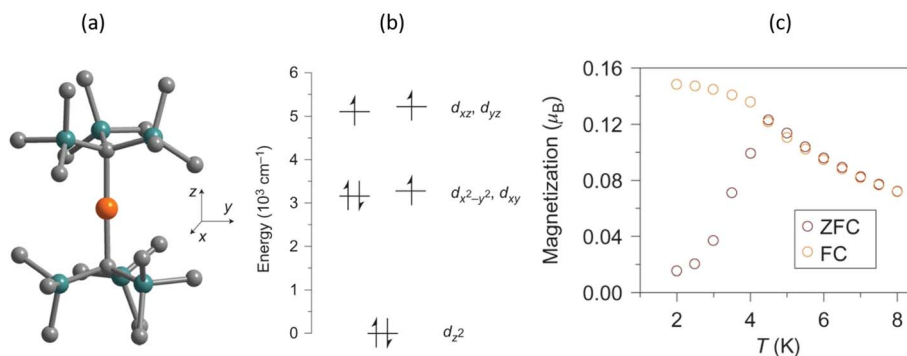
Fig. 2 Structure of [\text{FeC}(\text{C}(\text{SiMe}_3)_3)_2]^{1-} from the crystal structure of [\text{K}(\text{crypt-222})][\text{FeC}(\text{C}(\text{SiMe}_3)_3)_2] . Orange, turquoise and grey spheres represent Fe, Si and C, respectively (a). Energies of 3d molecular orbitals from ab initio ligand field CASSCF(NEVPT2) calculations (b). Low-temperature magnetisation data reveal blocking at 4.5 K, with divergence between field-cooled (FC) and zero-field-cooled (ZFC) measurements (c) (adapted from ref. 1 with permission of Nature Publishing Group, copyright 2013).
