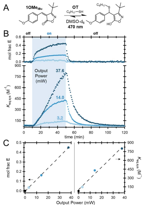
Fig. 5 (A) Equilibrium between 10Me_{tBu} and OT. (B) Mole fraction of the Z isomer and overall system K_{eq} ( K_{eq,sys} ) of 10Me_{tBu} equilibrated with OT during the NMR photoisomerization experiment at varying LED output powers (3.2 to 37.6 mW). (C) Mole fraction of Z isomer and maximum system K_{eq} versus LED output power.
