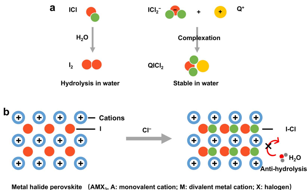
Fig. 5 Confining iodine through coordination chemistry. (a) Schematic diagram of the complexation of quaternary ammonium salts ( Q^+ ) with ICl_2^- in aqueous media. (b) Schematic illustration of iodine oxidation at perovskite type electrodes.
