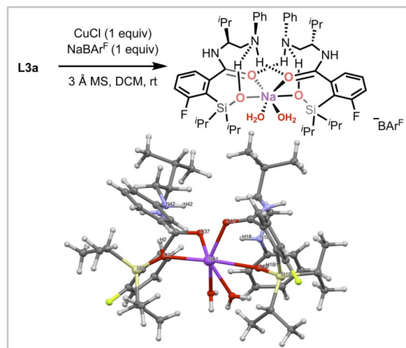
Fig. 4 Single-crystal structure of intermediate complex [(\mathbf{L3a})_2/\text{Na} \cdot (\text{H}_2\text{O})_2]^+[\text{BAR}^{\text{F}}]^- isolated from slow solvent evaporation over two months. The \text{BAR}^{\text{F}} anion has been omitted for clarity. Selected bond distances (Å), H-bonding interactions, and angles (deg): Si(2)-O(2): 1.634(4), Na(1)-O(2): 2.284(10), Na(1)-O(37): 2.441(8), O(2)-H(2)...N(42), N(18)-H(18)...O(37), N(42)-H(42)...O(13), O(1B)-H(1B1)...N(18), \angle Si(2)-O(2)-Na(1): 133.7(2).
