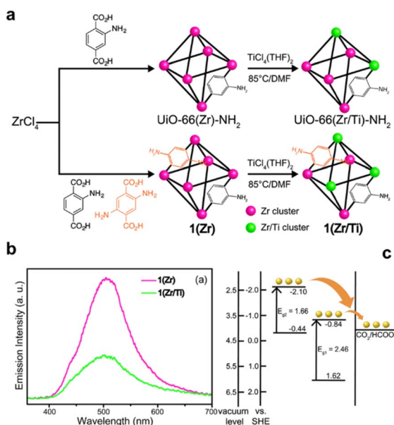
Fig. 11 (a) Synthesis of mixed-ligand MOF 1(\text{Zr}) via PSE to obtain mixed-metal MOFs 1(\text{Zr/Ti}) and \text{UiO-66}(\text{Zr/Ti})\text{-NH}_2 . (b) Photoluminescence spectra of 1(\text{Zr}) and 1(\text{Zr/Ti}) . (c) Energy band structure of 1(\text{Zr/Ti}) derived from UPS and F(R) results, showing that heterogeneous ligands create two energy levels within the MOF, potentially facilitating \text{CO}_2 catalysis. Reproduced with permission. 209 Copyright 2015, Royal Society of Chemistry.
