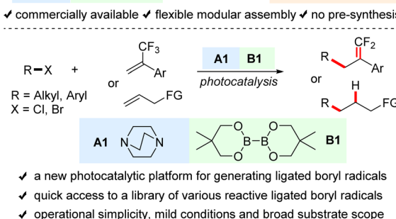
Scheme 1 (a) State-of-the-art of the cross-couplings via XAT by ligated boryl radicals. (b) This work.
