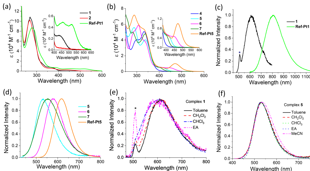
Fig. 2 Absorption spectra of (a) complexes 1 , 2 , and Ref-Pt 1 , (b) complexes 4–7 and Ref-Pt 5 in \text{CH}_2\text{Cl}_2 at RT. Emission spectra of (c) complexes 1 and Ref-Pt 1 , (d) complexes 5–7 and Ref-Pt 5 in deoxygenated \text{CH}_2\text{Cl}_2 ( 2 \times 10^{-5} \text{ M} ) at RT. Emission spectra of (e) complexes 1 and (f) 5 in various solvents. Asterisk (*) indicates Raman scattering of excitation light.
