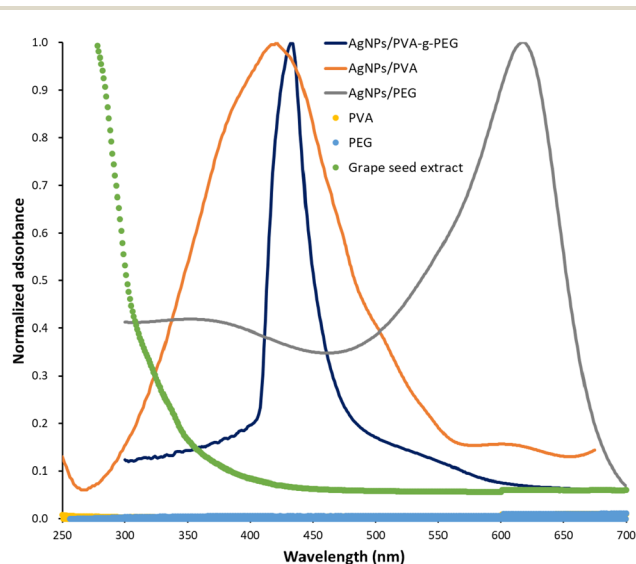
Fig. 3 UV-vis spectra of the AgNPs prepared from different polymers.
