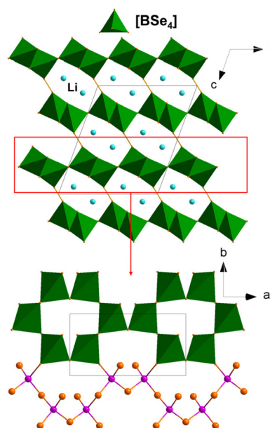
Fig. 11 The structure of \text{Li}_2\text{B}_2\text{Se}_5 .
