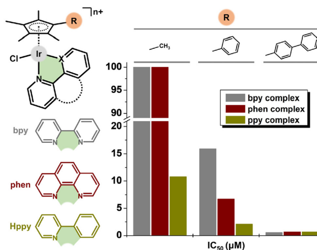
Fig. 31 The dependence of the in vitro antiproliferative activity of [Ir(η 5 -Cp x )Cl(L n ) n+ ] complexes in A2780 ovarian carcinoma cells on the cyclopentadienyl ring size; Cp x = Cp * , Cp bph or Cp bpy , L n = 2,2'-bipyridine (bpy; n = 1), 1,10-phenanthroline (phen; n = 1) or deprotonated 2-phenylpyridine (ppy; n = 0).
