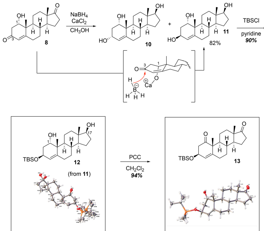
Scheme 3 Synthesis of 3-tert-butyldimethylsiloxy-1,17-diketo-androst-4-ene (13) from 1 \alpha -hydroxyandrostenedione (8) (Steps 3–5 of 8 steps). The intermediate in brackets explains the stereoselective reduction at C3 through the chelation of the calcium Lewis acid with the C1 \alpha -hydroxy group and the borohydride to deliver the hydride at the bottom face, yielding 11.
