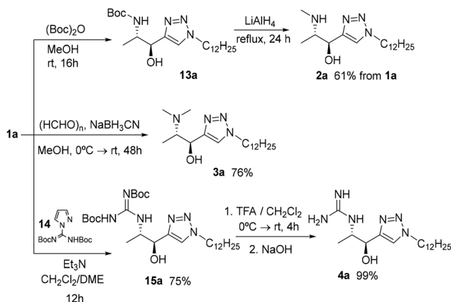
Scheme 5 Derivatisation of the amino moiety in 1a to give 1-deoxy-sphingolipid analogues 2a , 3a and 4a .
